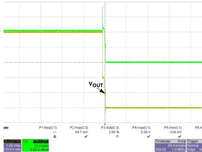
FIGURE 47. I O OVERSHOOT, SHORT @ V IN = 75V, I O = 40A
