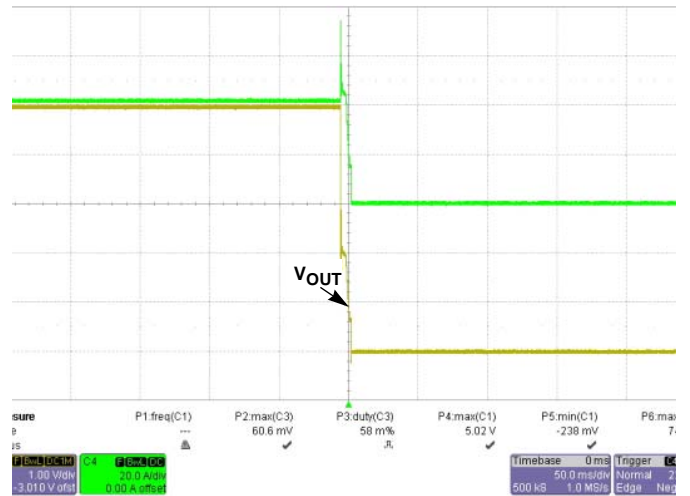
FIGURE 46. I O OVERSHOOT, SHORT @ V IN = 48V, I O = 40A
