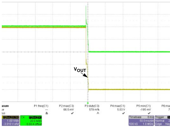
FIGURE 45. I O OVERSHOOT, SHORT @ V IN = 36V, I O = 40A
